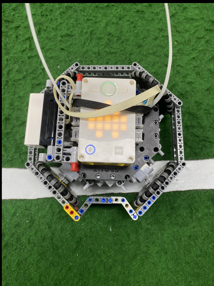
Image of our offensive robot
